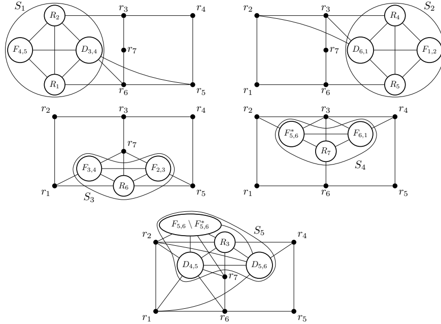
Figure 4: A 5-coloring of G \setminus (Z \cup D_{1,2}) when G contains a ruby. The picture shows the complement \overline{G} of G . A line between two sets does not necessarily mean that they are complete to each other in \overline{G} . Also some adjacency may be unrepresented. Each circled set is a clique in \overline{G} .
