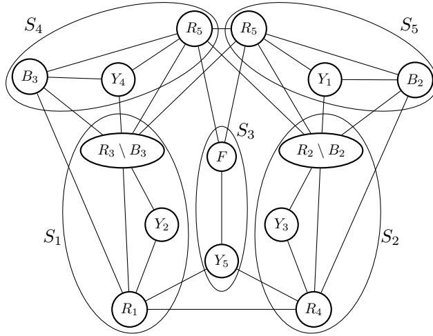
Figure 5: A 5-coloring of G \setminus Z when G contains a special solitaire (case 1). The picture shows the complement \bar{G} of G . A line between two sets does not necessarily mean that they are complete to each other in \bar{G} . Also some adjacency may be unrepresented. Each circled set is a clique in \bar{G} .
